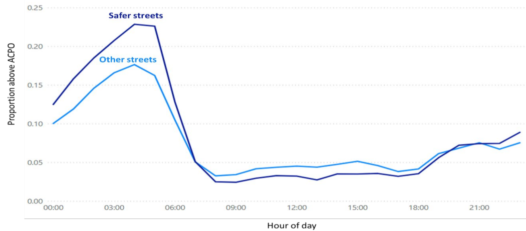
Figure 4.5: Visualisation of the variation in weekday proportion of observed vehicles travelling above the ACPO limit (10% plus 2mph above posted speed limit) averaged across all sampled weekdays by hour and by Safer Streets junction cluster
