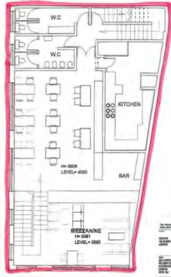
FIRST FLOOR - OPTION 1
