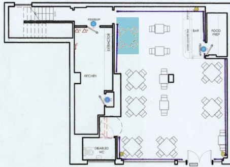
Proposed Ground Floor Plan 1:100
