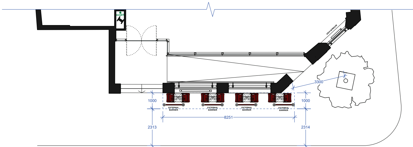
PROPOSED EXTERNAL SEATING PLAN
